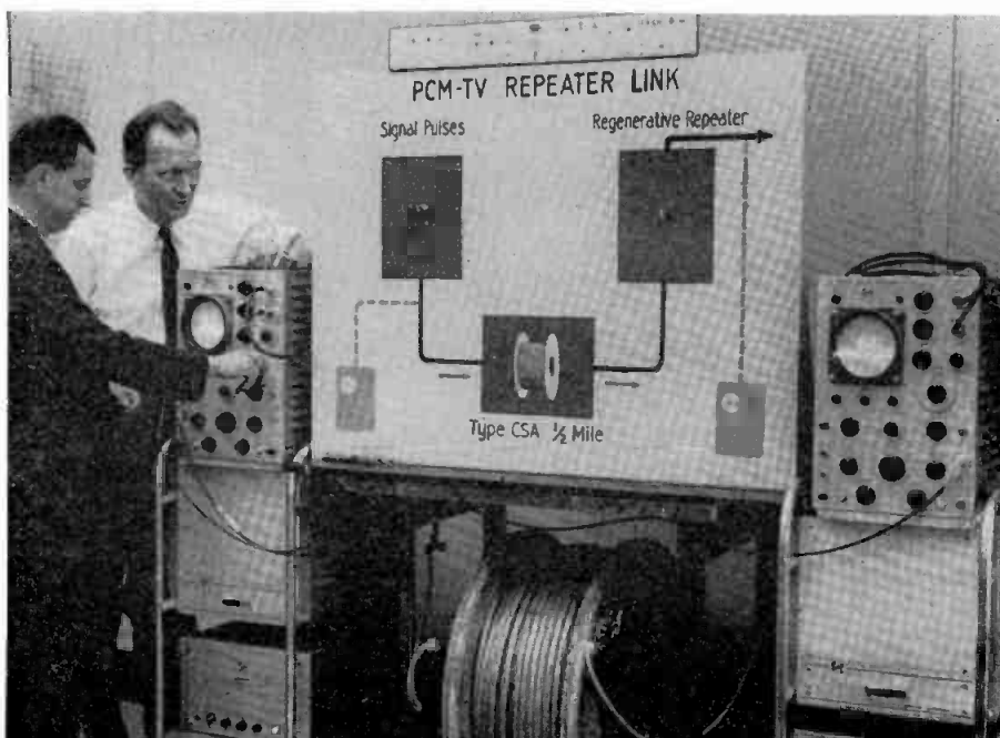
BELL LABS pulse-code modulation repeat links is demonstrated here by R. L. Carbrej (l) and A. J. Rack. Incoming pulses are shown both before (l) and after they have passed through a half-mile of cable and been amplified by a transistorized regenerative repeater.
